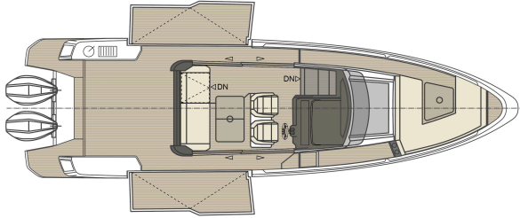
01 Main deck
